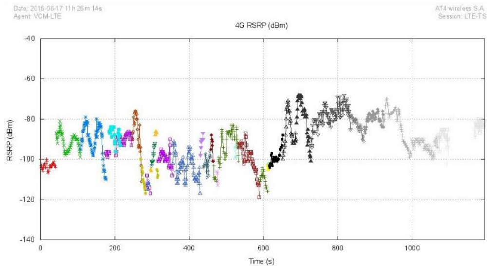
Figure 51: VCM RSRP
