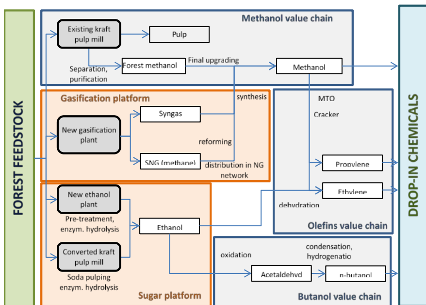
Figure 2 Overview of Skogskemi platforms and value chains
